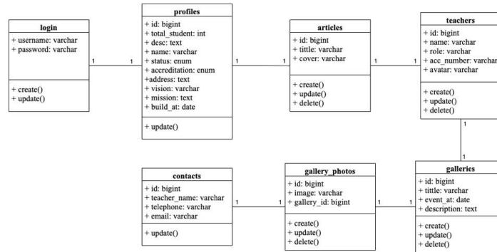
Gambar 4. 2 Class Diagram Usulan
