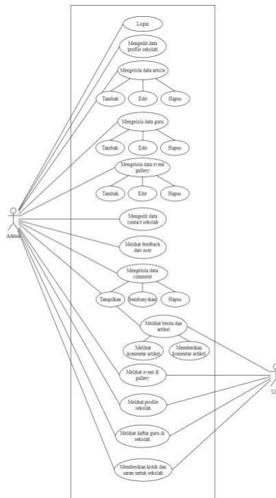
Gambar 4. 1 Usecase Diagram Usulan
